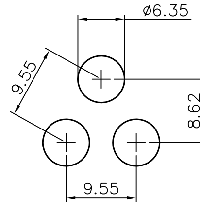
Enlarged Detail
