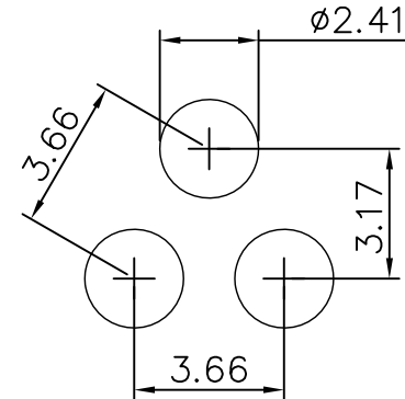
Enlarged Detail
